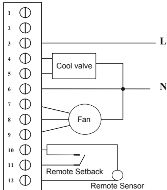
Typical wiring for ON/OFF control in 2 pipe cooling only (VC6013)
