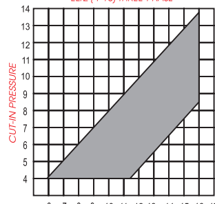
CUT-OUT PRESSURE
