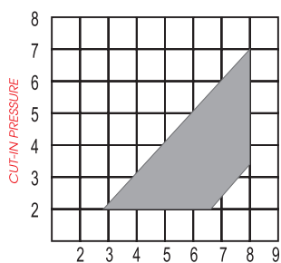
CUT-OUT PRESSURE
